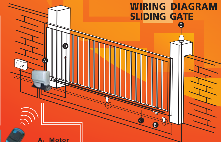
A: Motor B: Limit stopper or Limit magnet C: Rack D: Photocell E: Flashing Lamp
